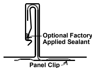
Seam Profile
